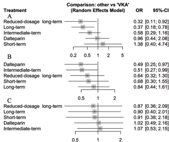
Figure 2. Direct comparisons of DOAC strategies in cancer-associated thrombosis. (A) Recurrent VTE; (B) Major bleeding; (C) All-cause mortality.
