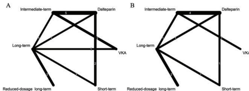
Figure 1. Network diagrams of included studies. (A) Recurrent VTE and major bleeding; (B) All-cause mortality.
