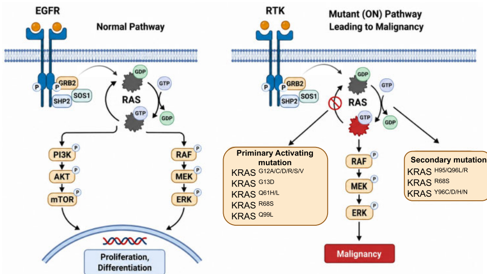
Figure 1. KRAS signaling and mechanisms of oncogenic activation and acquired resistance. RAF, rapidly accelerated fibrosarcoma; MEK, mitogen-activated protein kinase kinase; ERK, extracellular signal-regulated kinase; PI3K, phosphoinositide 3-kinase; AKT, protein kinase B; mTOR, mechanistic target of rapamycin; KRAS, Kirsten rat sarcoma viral oncogene homolog.
